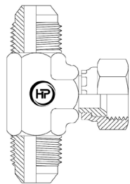
JICM X JICM X JICF BRANCH TEE
