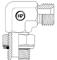
BSPPM X BSPPM 90° ELBOW (M X M)
