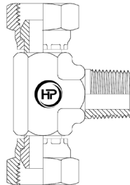
BSPPF X BSPPF X BSPTM BRANCH TEE
