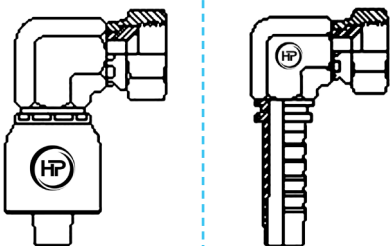
BSPF FEMALE SWIVEL 90° COMPACT
