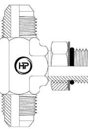
JICM X JICM X UNOM BRANCH TEE
